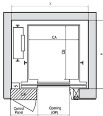
HOISTWAY PLAN
